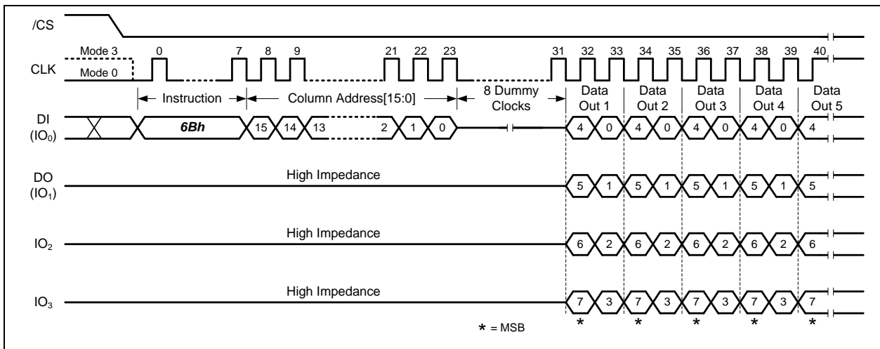
Figure 8-29 Fast Read Quad Output Instruction (Buffer Read Mode, BUF=1)
