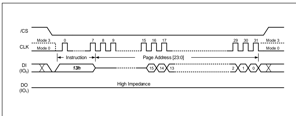
Figure 15. Page Data Read Instruction
