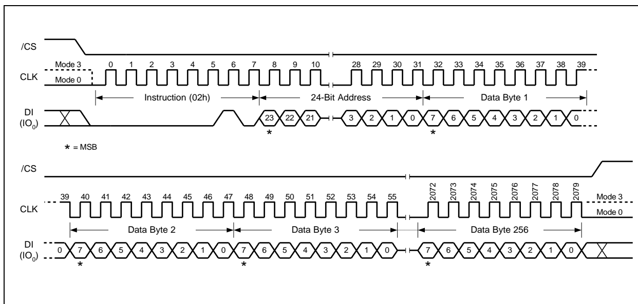
Figure 32. Page Program Instruction
