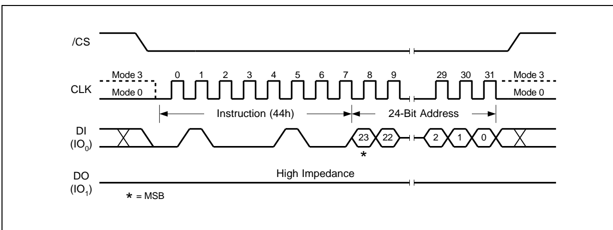
Figure 45. Erase Security Registers Command (SPI Mode only)
