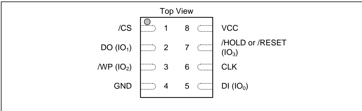
Figure 1b. W25Q32JW Pad Assignments, 8-pad SON 6x5-mm (Package Code ZP, XG, XH , UU)
