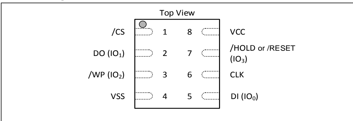
Figure 1b. W25Q32RV Pad Assignments, 8-pad WSON 6x5-mm, USON 2X3-mm (Package Code ZP, XH,UU)
