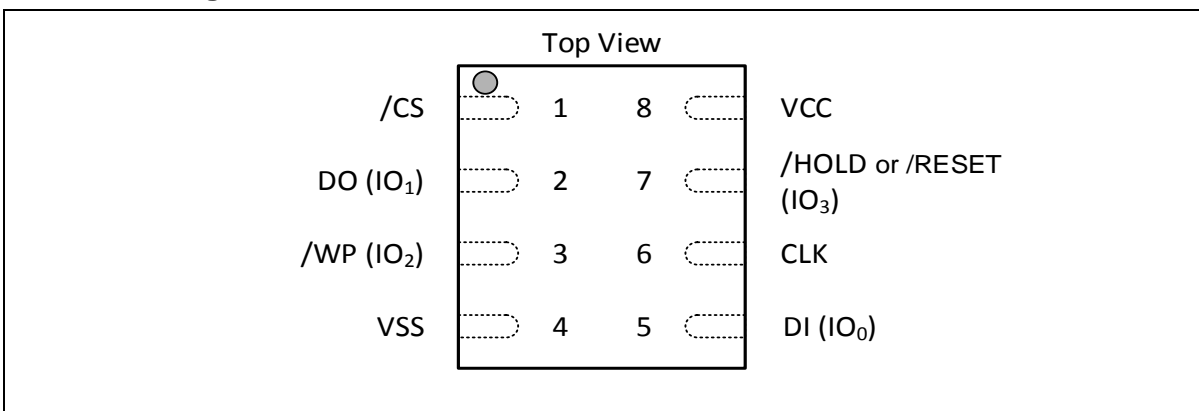
Figure 1b. W25Q32RV Pad Assignments, 8-pad XSON 2X3, WSON 6x5-mm (Package Code XH, ZP, UU)
