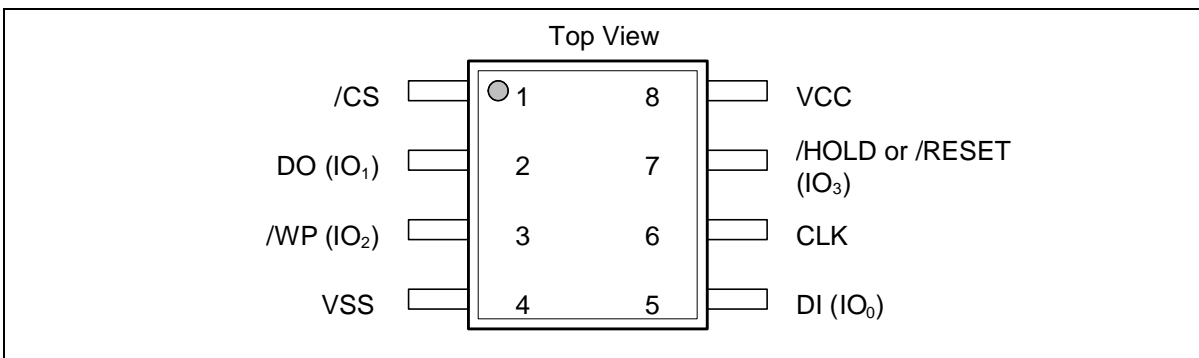
Figure 1a. W25Q32RV Pin Assignments, 8-pin SOP 150/208-mil (Package Code SN, SS)
