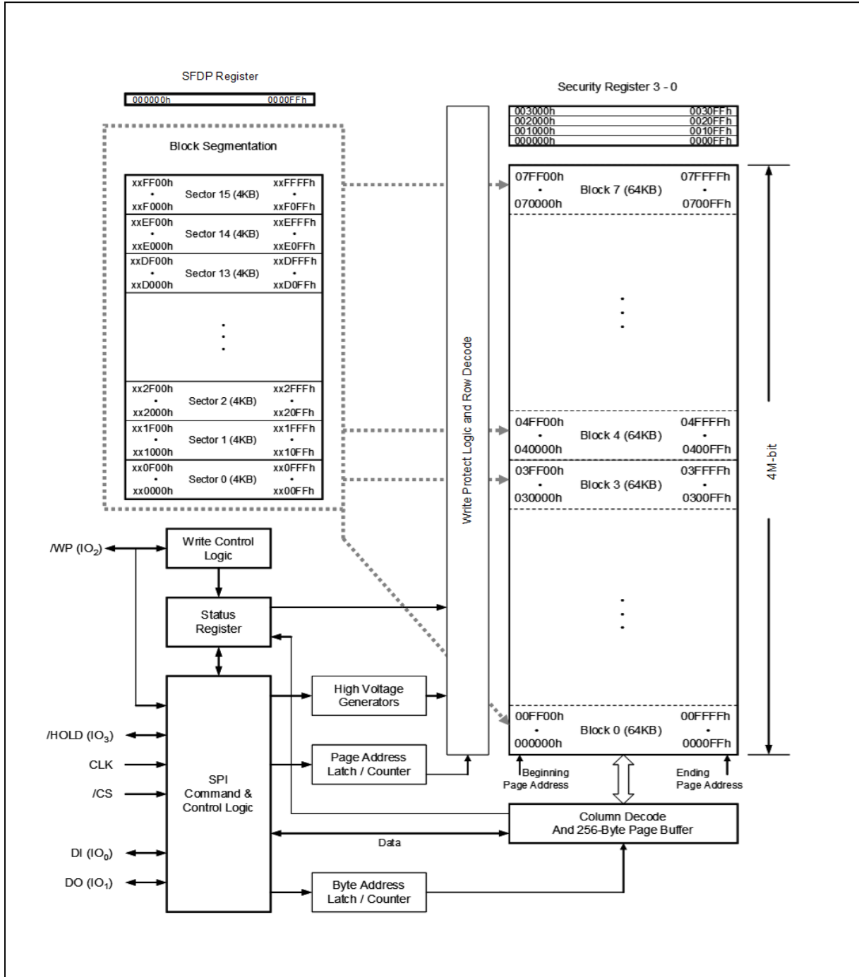
Figure 2. W25Q40RV Serial Flash Memory Block Diagram
