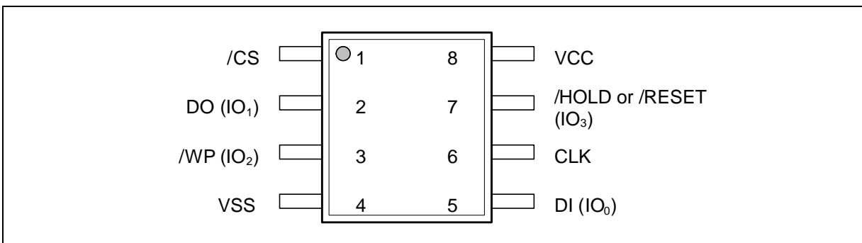
Figure 1a. Pin Assignments, 8-pin SOIC 150/208-MIL (Package Code SN, SS)
