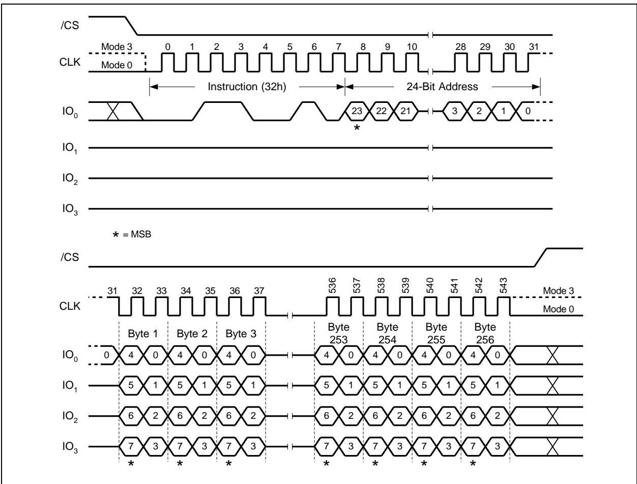
Figure 35. Quad Input Page Program Instruction (SPI Mode only) 32-Bit Address is required when the device is operating in 4-Byte Address Mode
