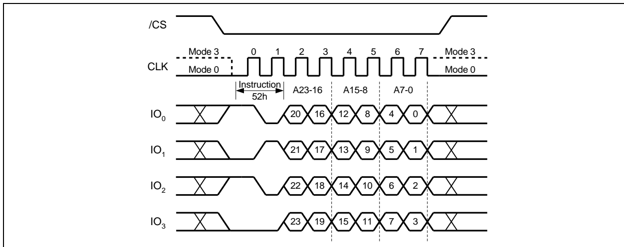
Figure 38b. 32KB Block Erase Instruction (QPI Mode) 32-Bit Address is required when the device is operating in 4-Byte Address Mode
