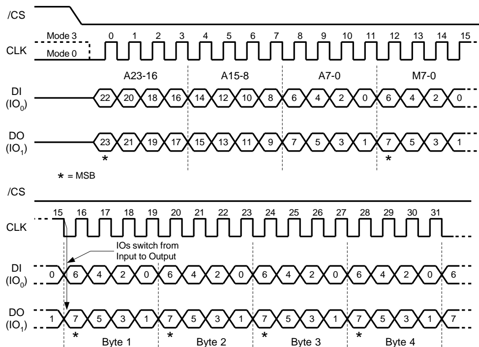
Figure 23b. Fast Read Dual I/O (Previous instruction set M5-4=10, SPI Mode only)
