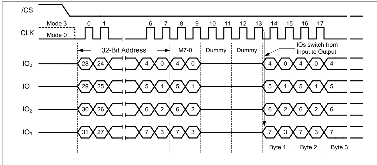
Figure 28b. Fast Read Quad I/O w/ 4-Byte Addr. (Previous instruction set M5-4=10, SPI Mode only)
