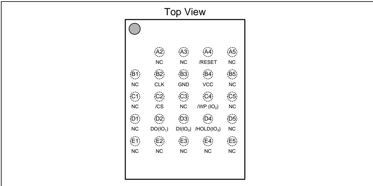
Figure 1d. W25Q64JV Ball Assignments, 24-ball TFBGA 8x6-mm (Package Code TB)
