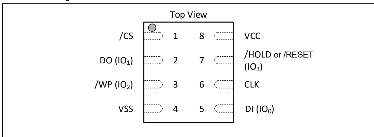
Figure 1b. Pad Assignments, 8-pad WSON 6x5-mm, XSON 2X3-mm (Package Code ZP & XH)
