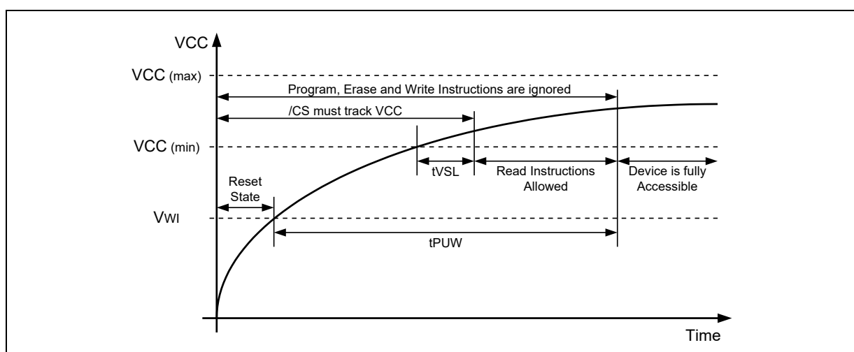
Figure 70a. Power-up Timing and Voltage Levels
