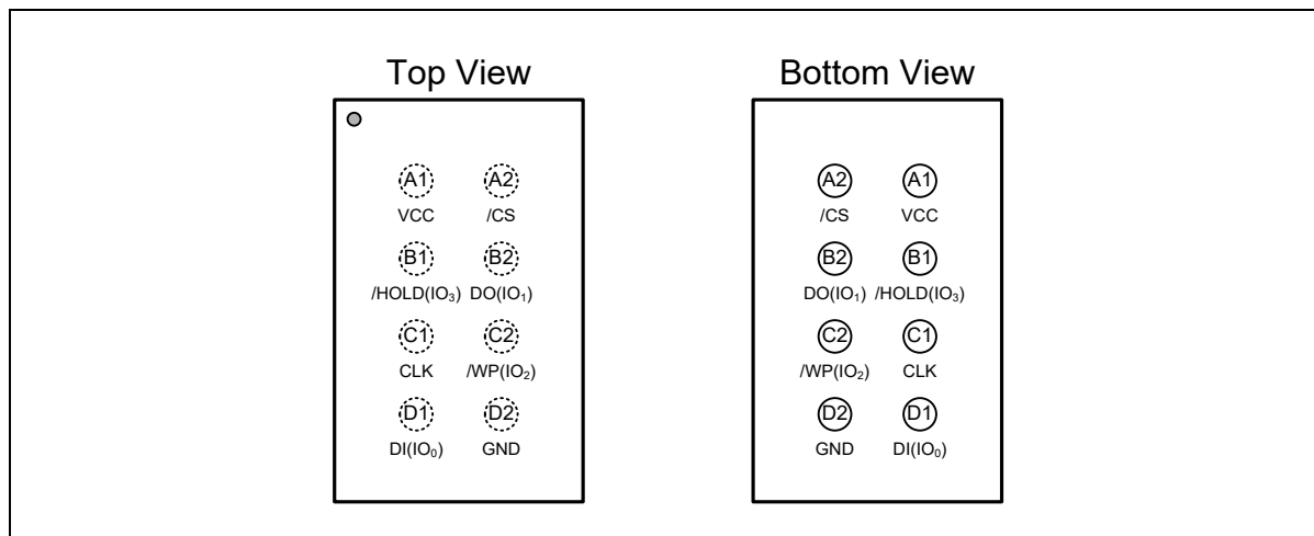
Figure 1c. W25Q80RV Ball Assignments, 8-ball WLCSP (Package Code BY)
