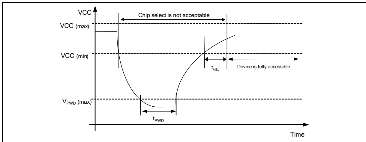
Figure 70c. Power Cycle Requirement
