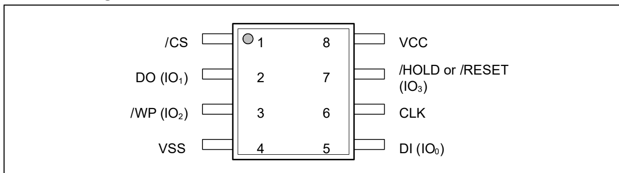
Figure 1a. Pin Assignments, 8-pin SOP 150/208-MIL (Package Code SN, SS)
