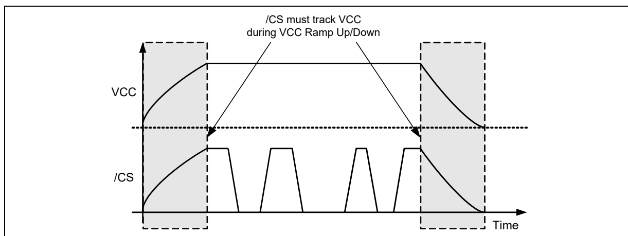
Figure 70b. Power-up, Power-Down Requirement
