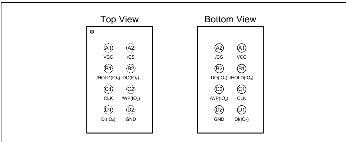
Figure 1c. W25QRV Ball Assignments, 8-ball WLCSP (Package Code BY)
