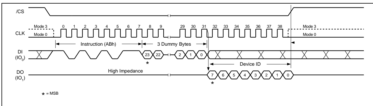
Figure 27b. Release Power-down / Device ID Instruction
