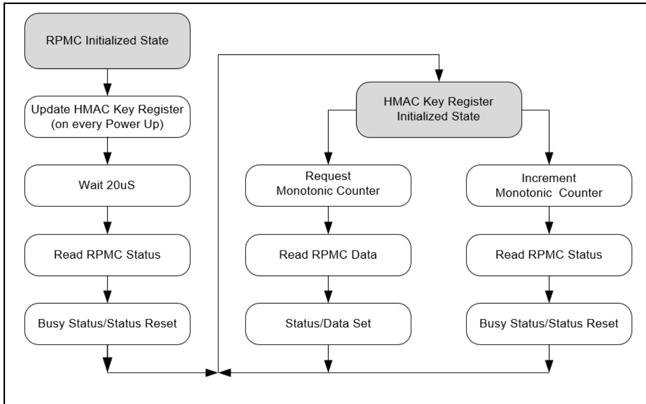
Figure 3b. W25R512JV RPMC Operation Flow Diagram
