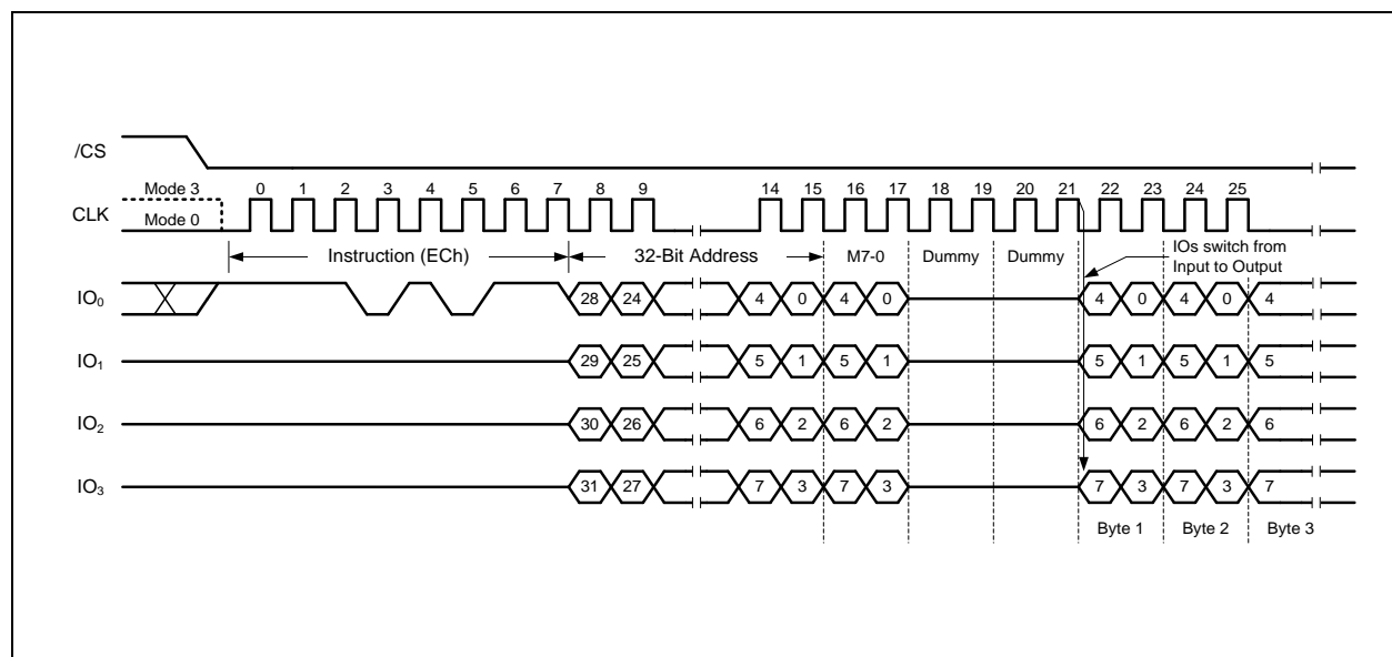
Figure 25a. Fast Read Quad I/O with 4-Byte Address Instruction (Initial instruction or previous M7-0 = Fxh)
