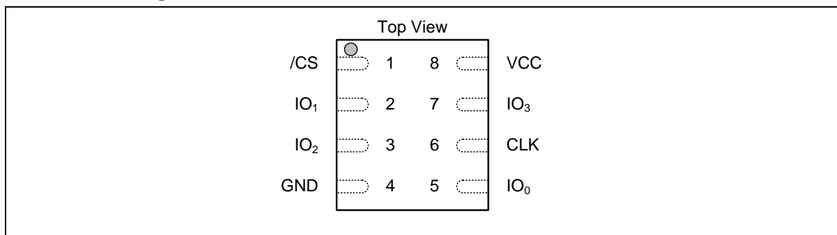
Figure 1a. W25R512JV Pad Assignments, 8-pad WSON 8x6-mm (Package Code E)
