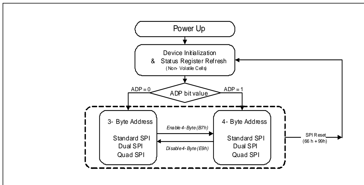
Figure 3. W25R512JV Serial Flash Memory Operation Diagram
