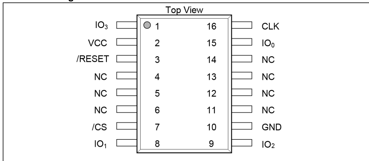
Figure 1d. W25R512JV Pin Assignments, 16-pin SOIC 300-mil (Package Code F)
