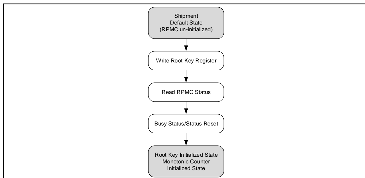
Figure 3a. W25R512JV RPMC Initialization Flow Diagram
