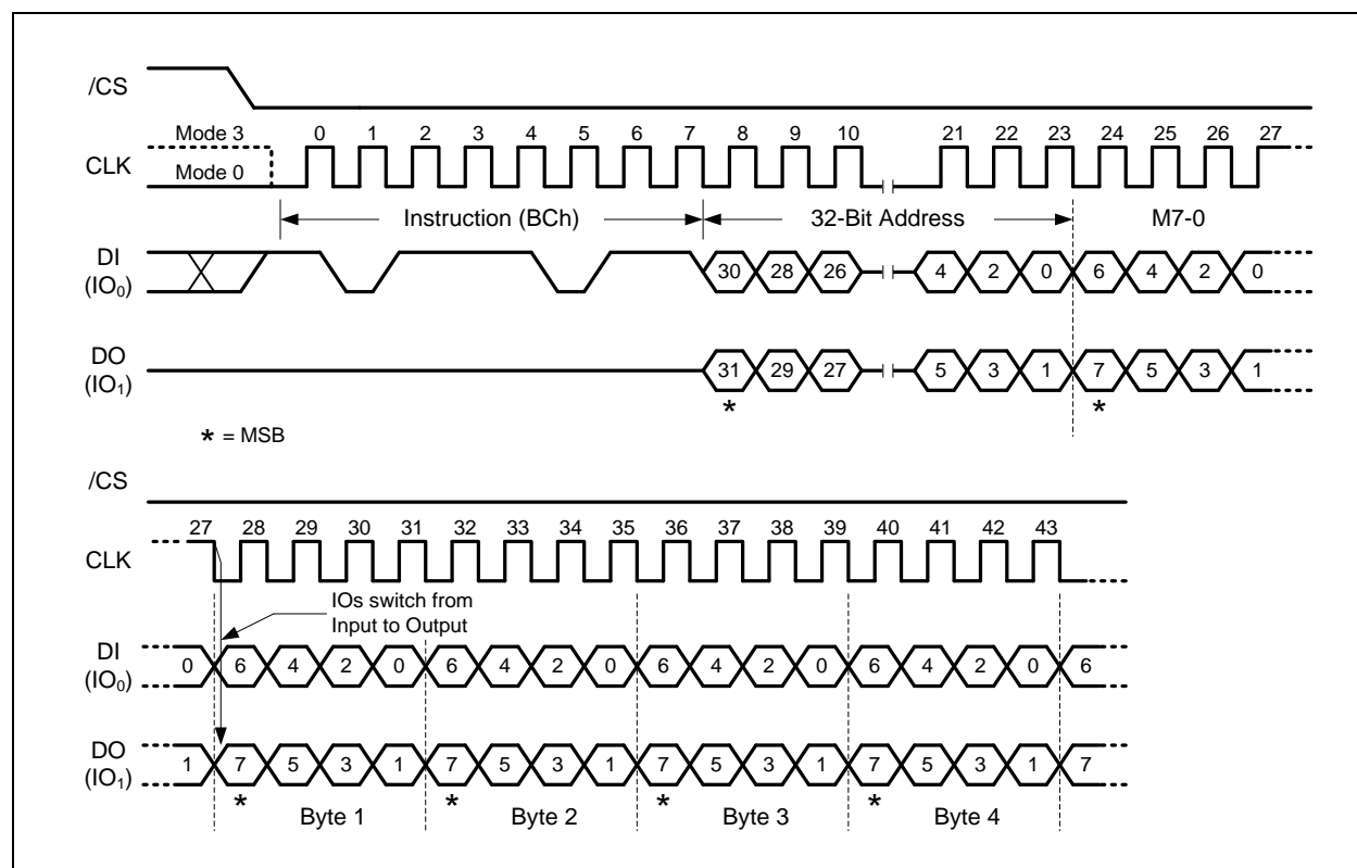
Figure 23a. Fast Read Dual I/O with 4-Byte Address Instruction (Initial instruction or previous M7-0 = Fxh)
