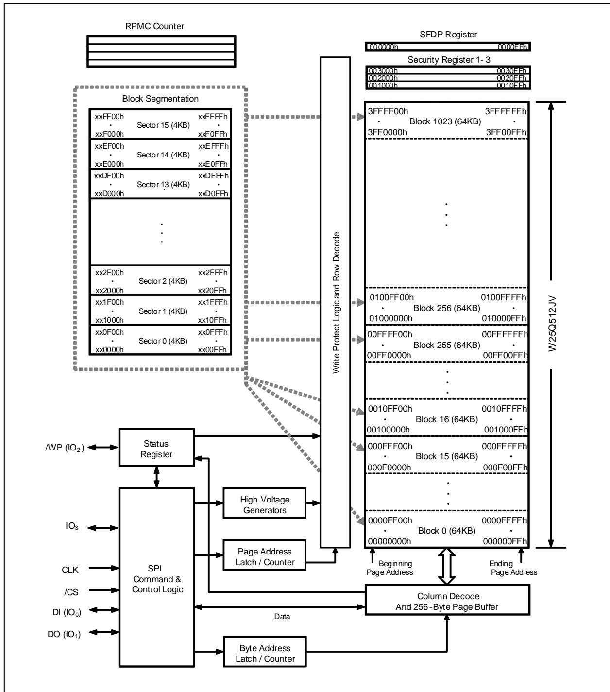
Figure 2. W25R512JV Serial Flash Memory Block Diagram
