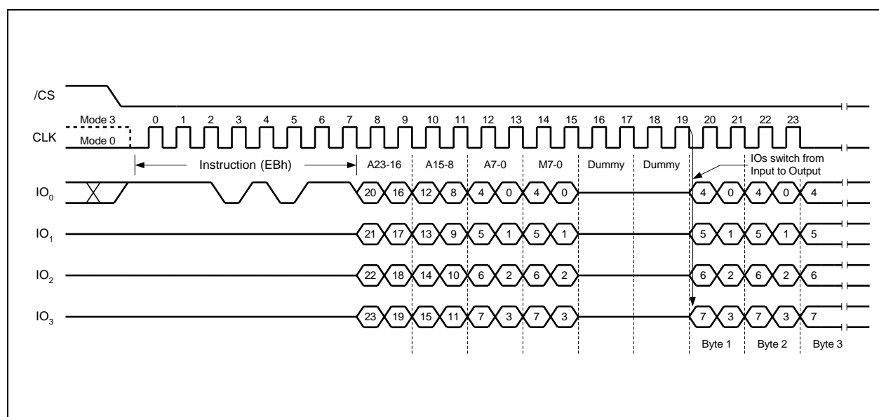
Figure 24a. Fast Read Quad I/O Instruction (Initial instruction or previous M7-0 = Fxh)
