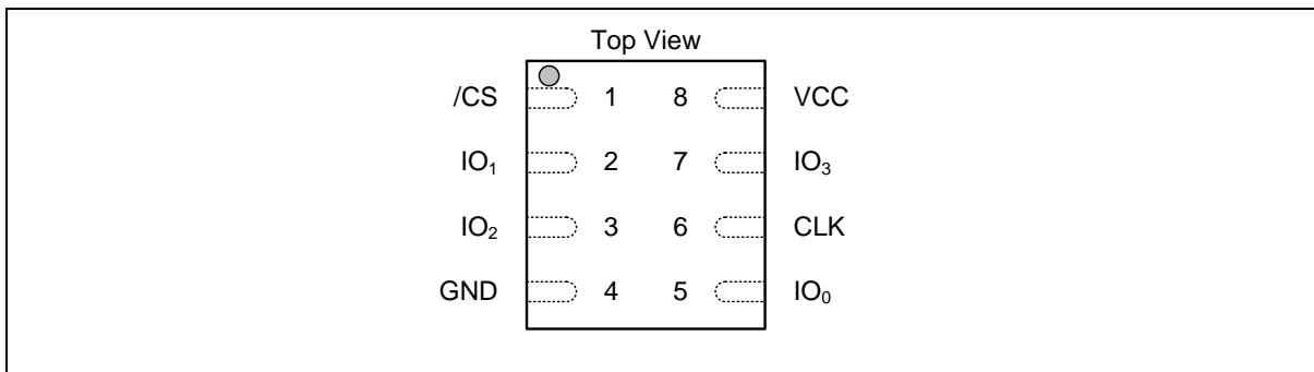
Figure 1b. W25R64JV Pad Assignments, 8-pad WSON 6x5-mm (Package Code ZP)
