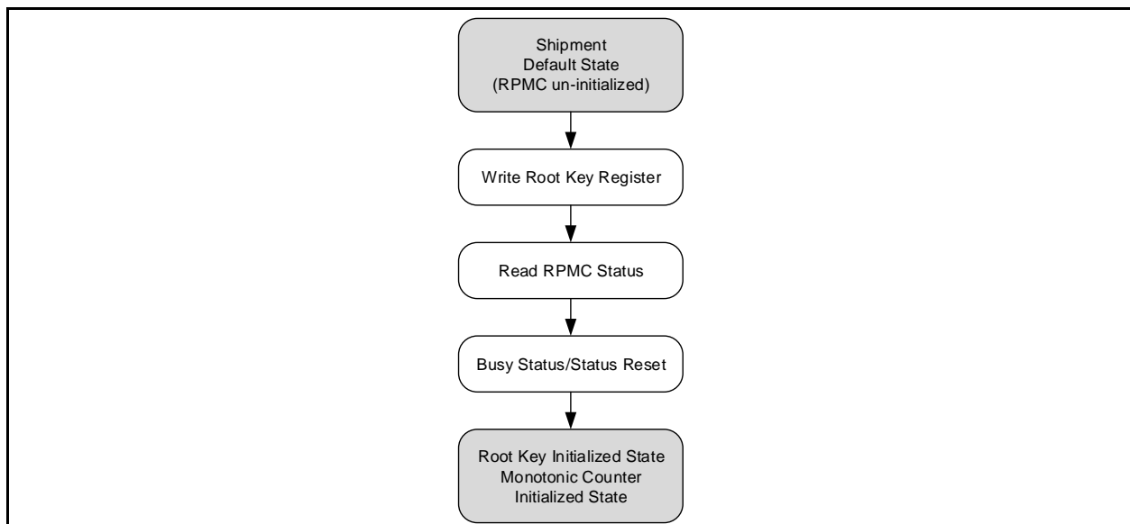
Figure 3a. W25R256JV RPMC Initialization Flow Diagram
