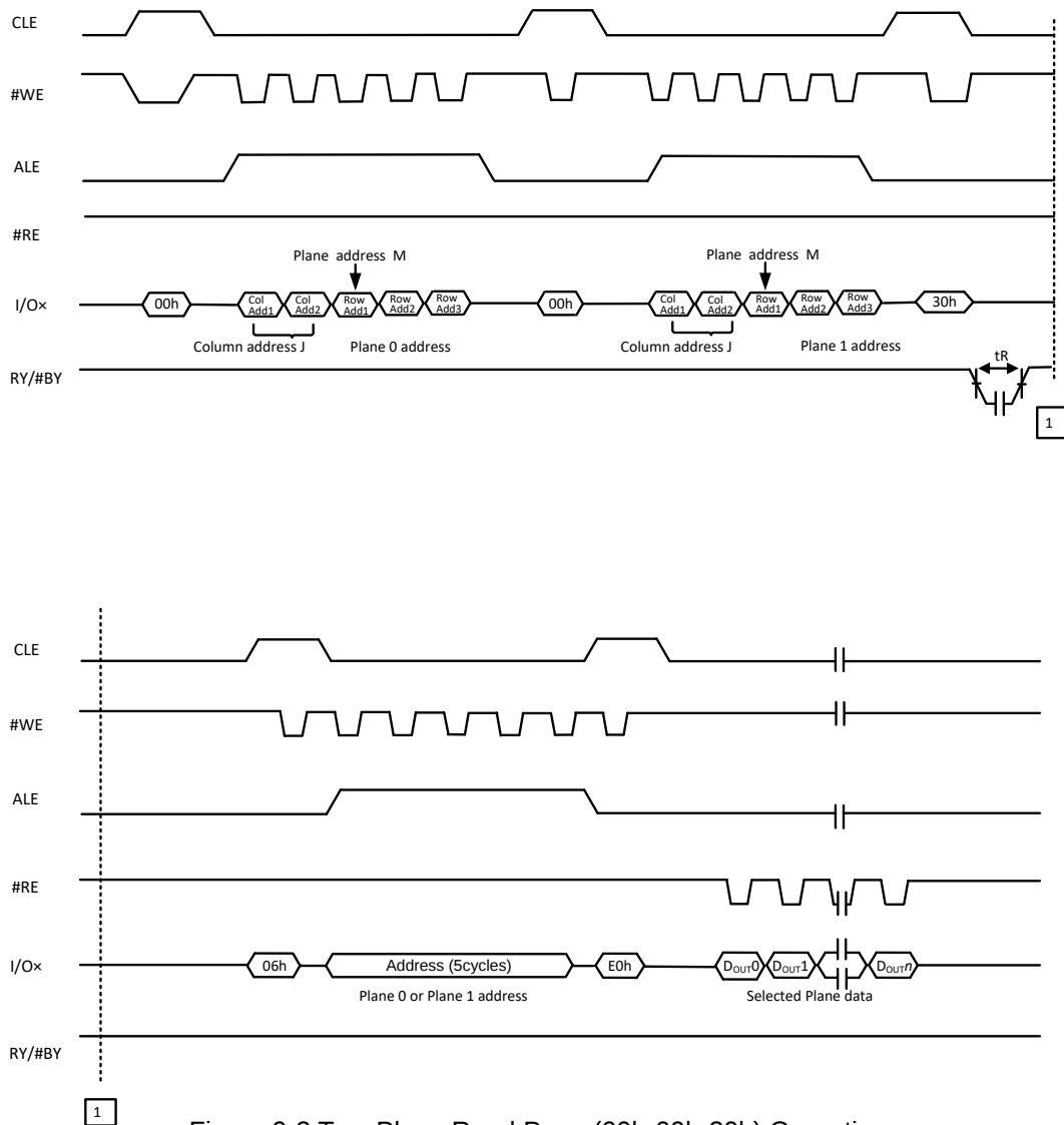
Figure 9-2 Two Plane Read Page (00h-00h-30h) Operation
