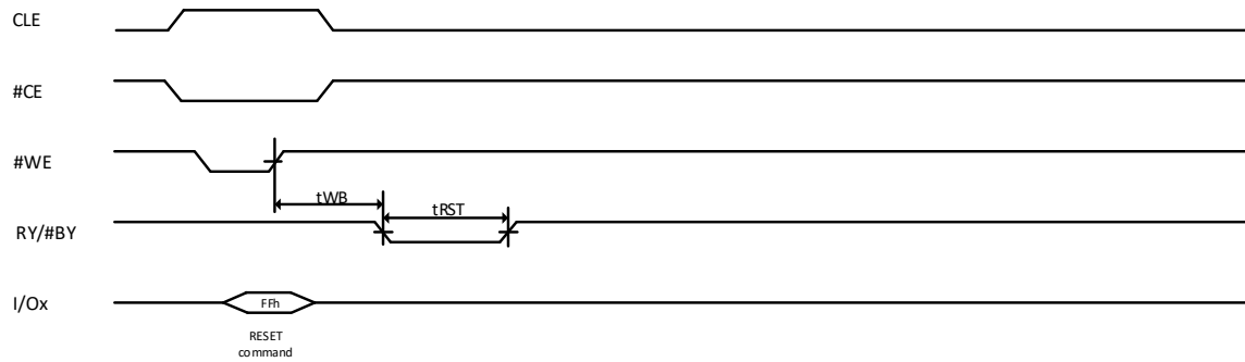
Figure 11-16 Reset
