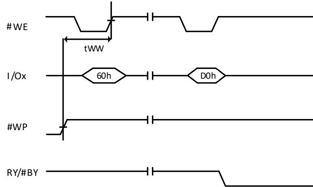
Figure 9-23 Erase Enable
