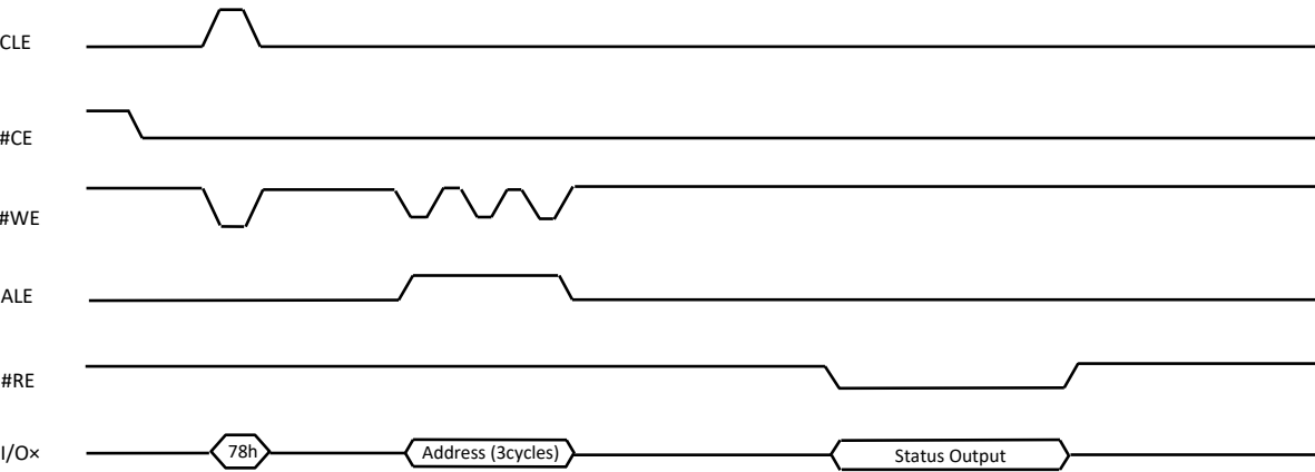
Figure 9-11 Read Status Enhanced (78h) Operation
