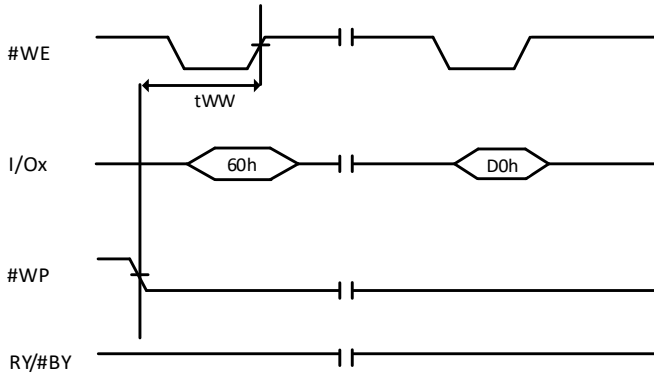
Figure 9-30 Erase Disable
