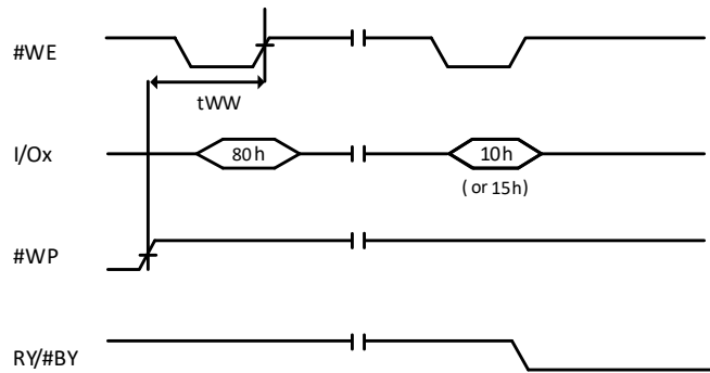
Figure 9-31 Program Enable
