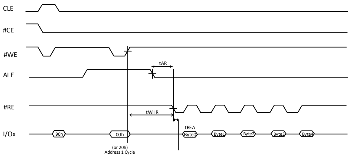
Figure 9-8 Read ID
