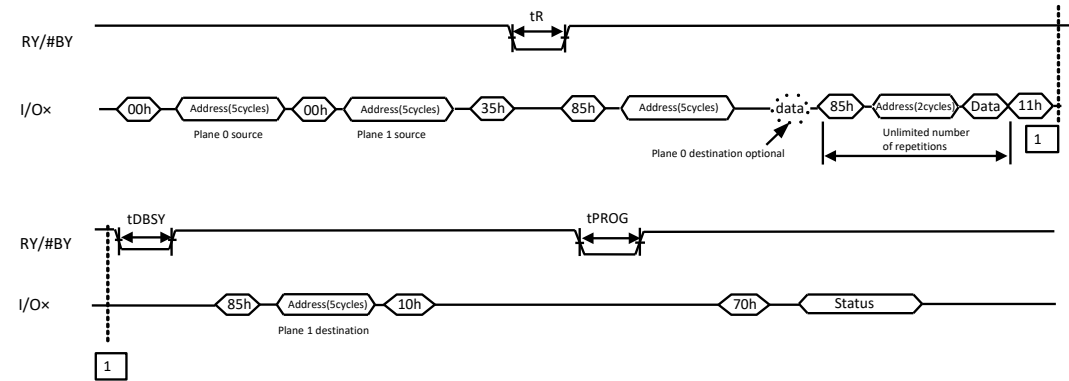
Figure 9-22 Two Plane Copy Back with Random Data Input
