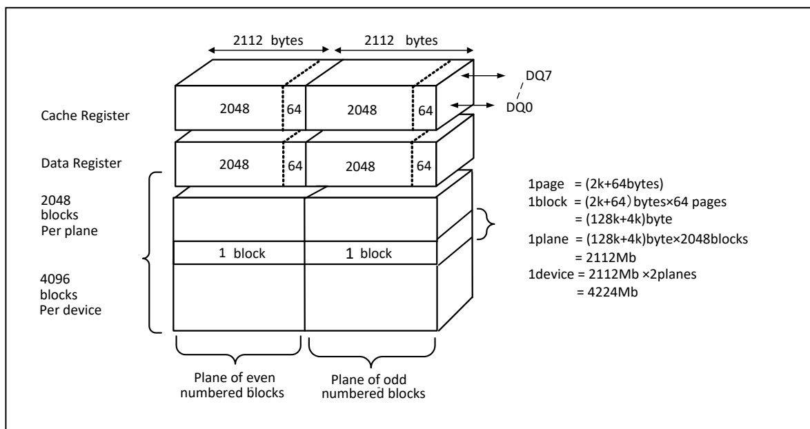
Figure 6-1 Array Organization
