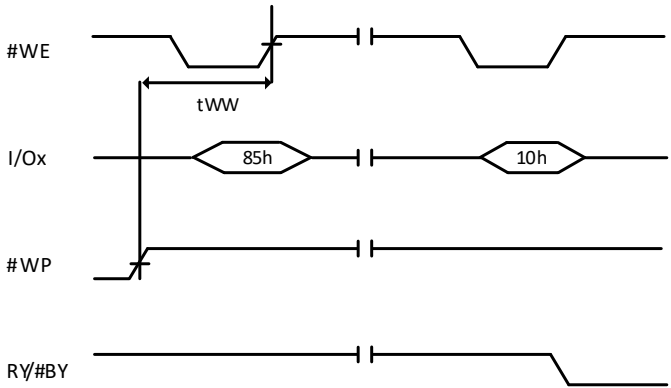
Figure 9-33 Program for Copy Back Enable
