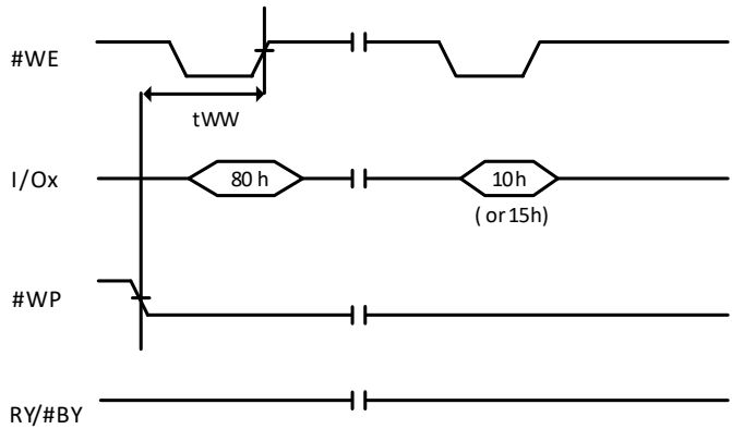
Figure 9-32 Program Disable
