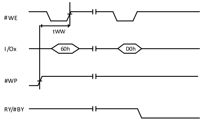
Figure 9-29 Erase Enable
