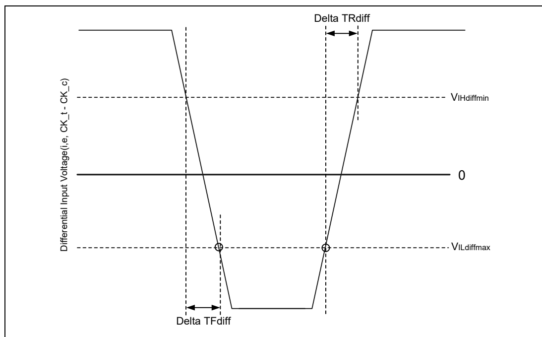
Figure 187 – Differential Input Slew Rate Definition for CK t , CK c
