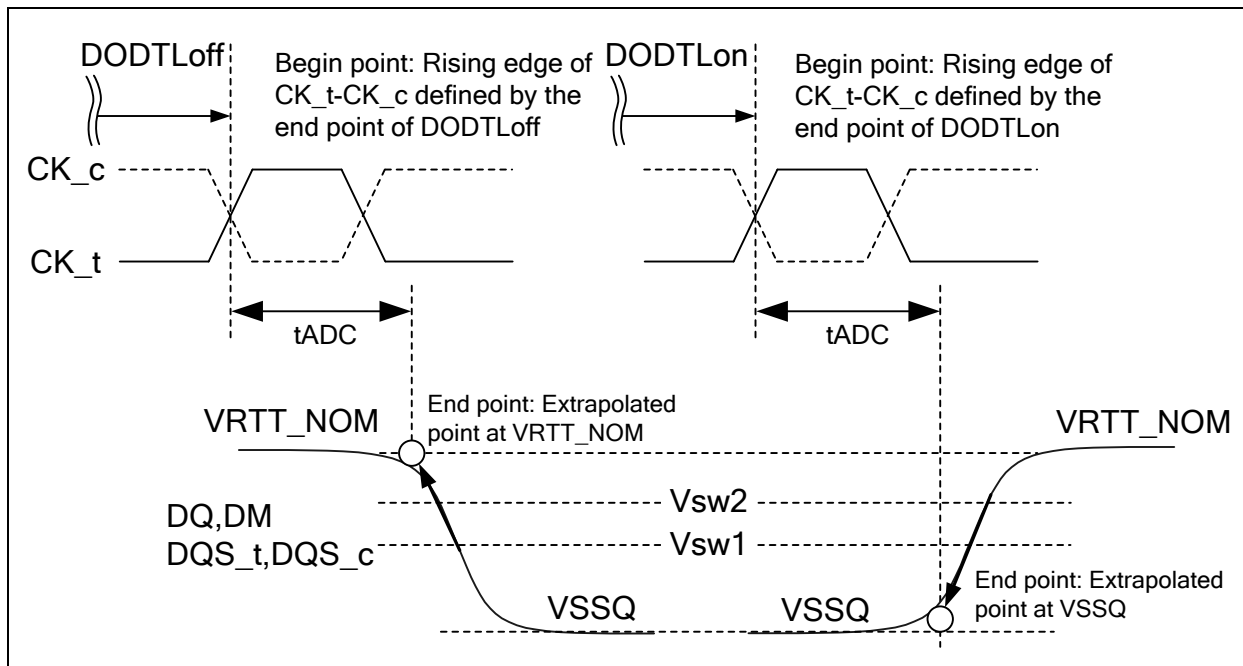
Figure 178 – Definition of t_{ADC} at Direct ODT Control
