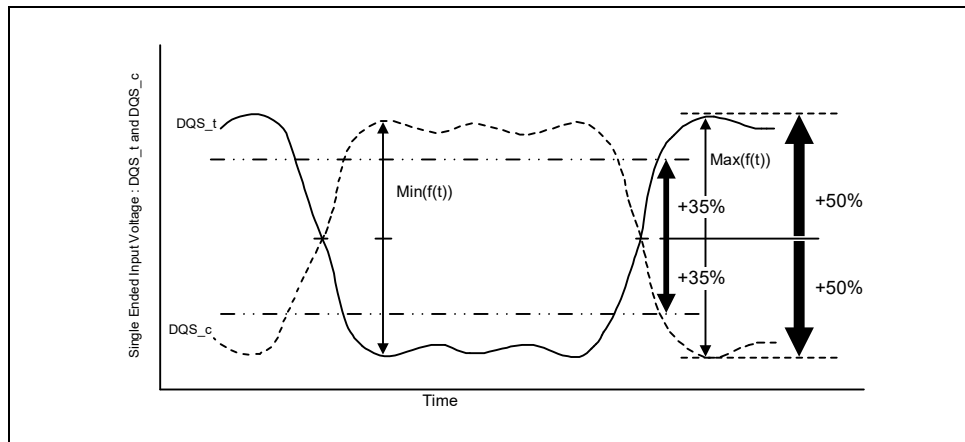
Figure 192 – Definition of differential DQS Peak Voltage and rage of exempt non-monotonic signaling
