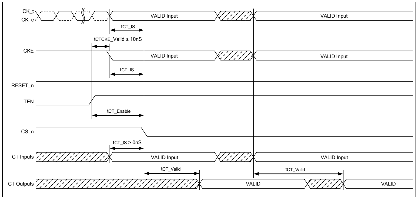
Figure 159 – Timing Diagram for Connectivity Test (CT) Mode
