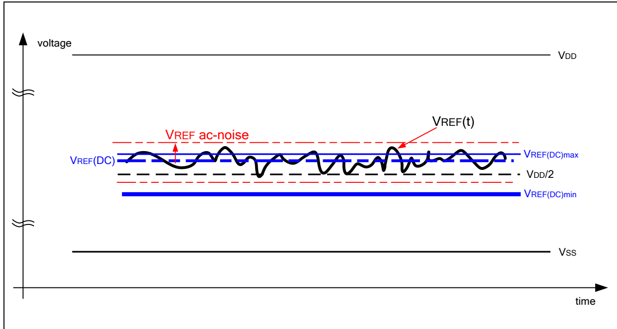
Figure 181 – Illustration of VREF(DC) tolerance and VREF AC-noise limits
