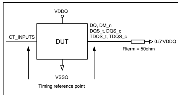
Figure 199 – Connectivity Test Mode Timing Reference Load
