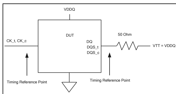
Figure 202 – Reference Load for AC Timing and Output Slew Rate
