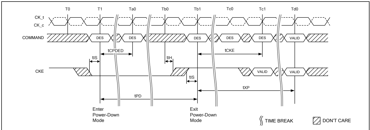
Figure 148 – Precharge Power-Down Entry and Exit
