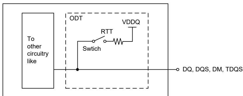
Figure 166 – Functional Representation of ODT
