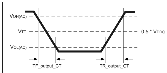
Figure 198 – Output Slew Rate Definition of Connectivity Test Mode
