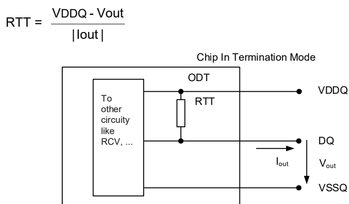
Figure 167 – On Die Termination
