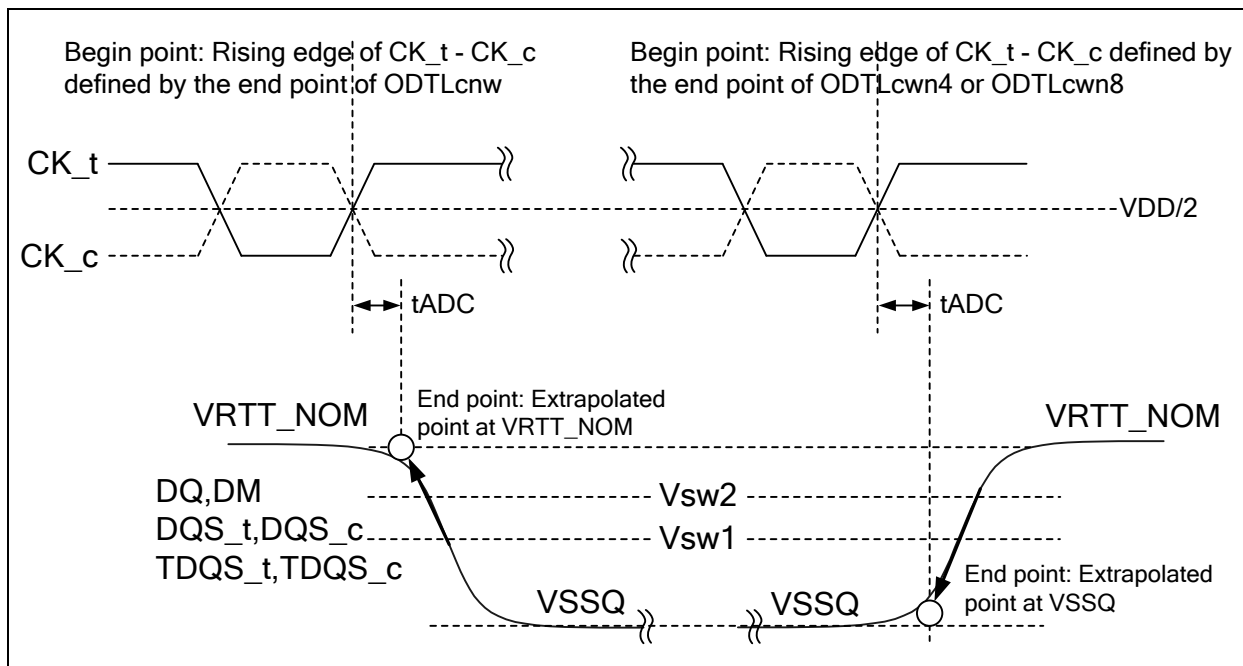
Figure 179 – Definition of t_{ADC} at Dynamic ODT Control
