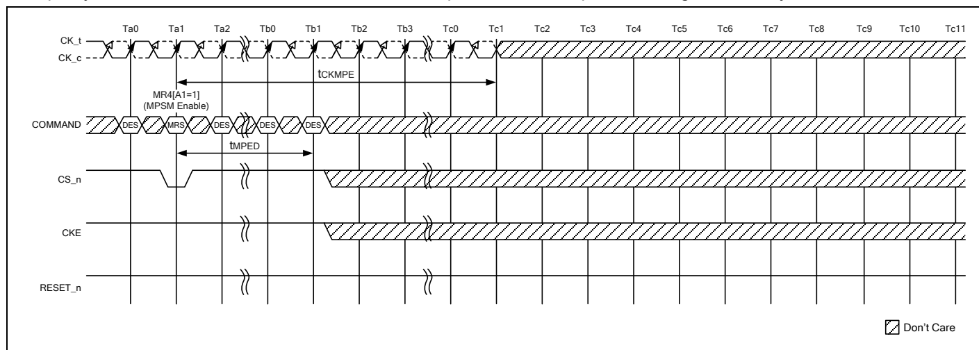
Figure 155 – Maximum Power Saving mode Entry
