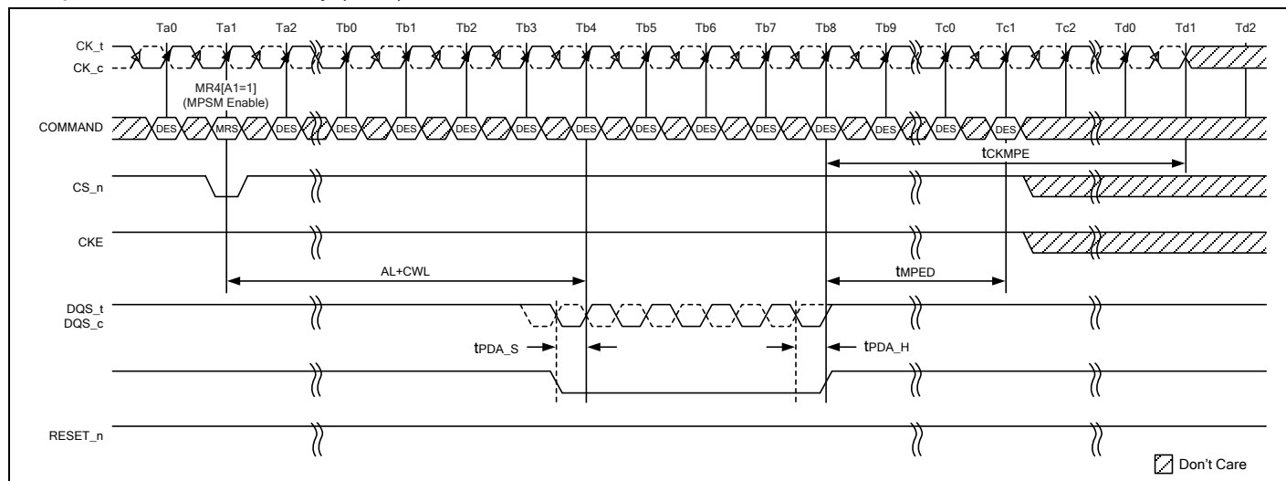
Figure 156 – Maximum Power Saving mode Entry with PDA
