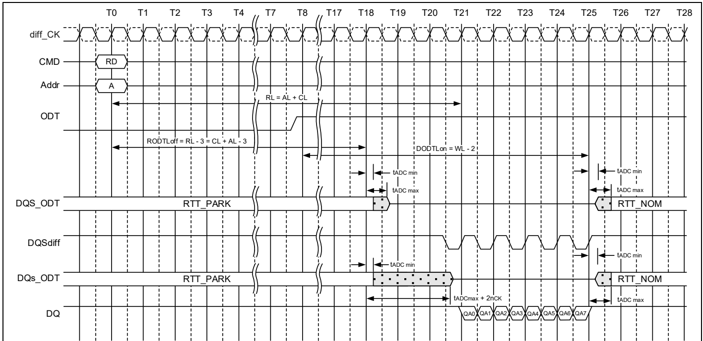
Figure 171 – Example: CL=11, PL=0; AL=CL-1=10; RL=AL+PL+CL=21; CWL=9; DODTLon=AL+CWL-3=17; RODTLoft=CL+AL-3=18; 2tCK preamble
