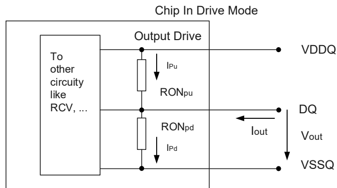
Figure 195 – Output driver
