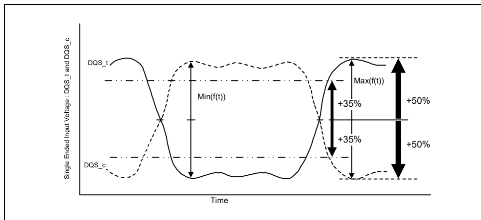
Figure 192 – Definition of differential DQS Peak Voltage and range of exempt non-monotonic signaling
